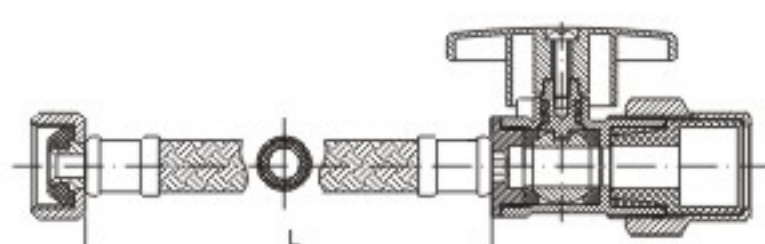
KLOE8131 F1/2"x1/2"CPVC Valve stop
