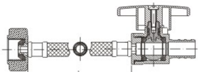
KLOE825H F7/8"BCx1/2"PEX Valve stop
