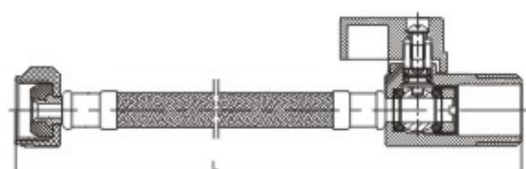
KLOE8133J G1/2"x1/2"Ball Valve
