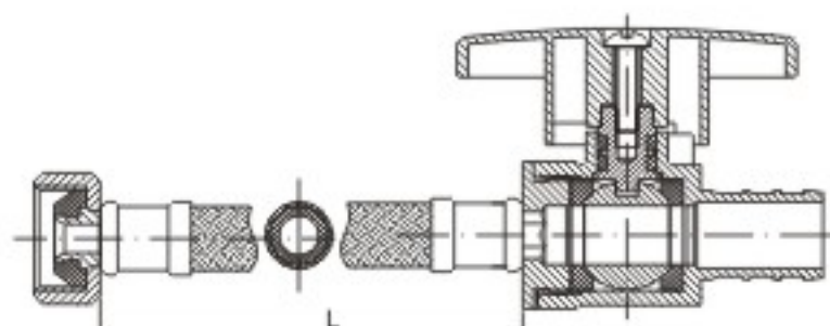
KLOE813H F1/2"x1/2"PEX Valve stop
