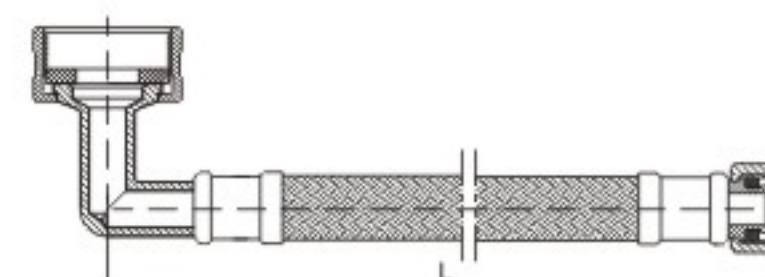
KLOE811F F3/8"C×F3/4"Elbow
