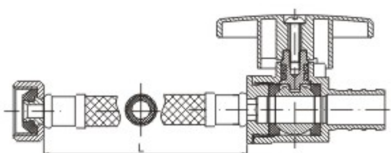
KLOE823H F1/2"x1/2"PEX Valve stop
