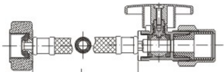
KLOE825I F7/8"BCx1/2"CPVC Valve stop
