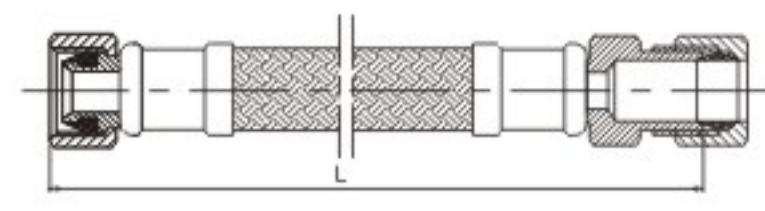
KLOE8119 F3/8"C×M·F3/8"C
