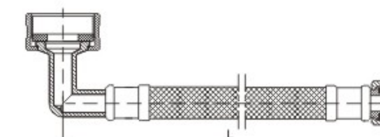
KLOE821F F3/8"C×F3/4"Elbow
